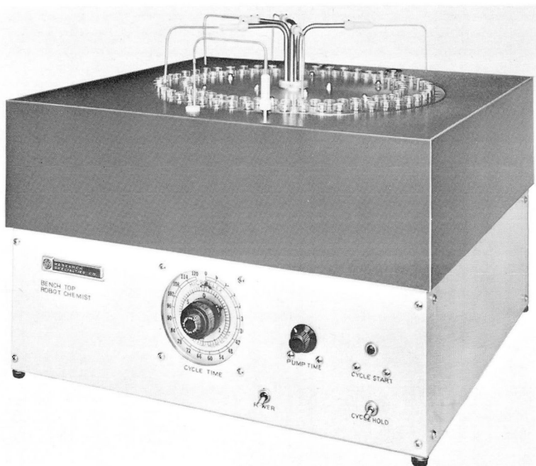
Fig. 14. Bench-Top Robot Chemist. All working parts are contained within the cabinet; turn-table and transfer pipets project above; complicated analysis may require two or more units placed side by side; colorimetric system is not shown. (Courtesy of Research Specialties Company, Richmond, California.)
