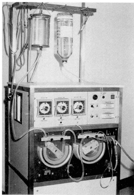
Fig. 3. Drake-Willock automatic peritoneal dialysis machine. This unit contains a reverse osmosis water purification system and proportioning system.
