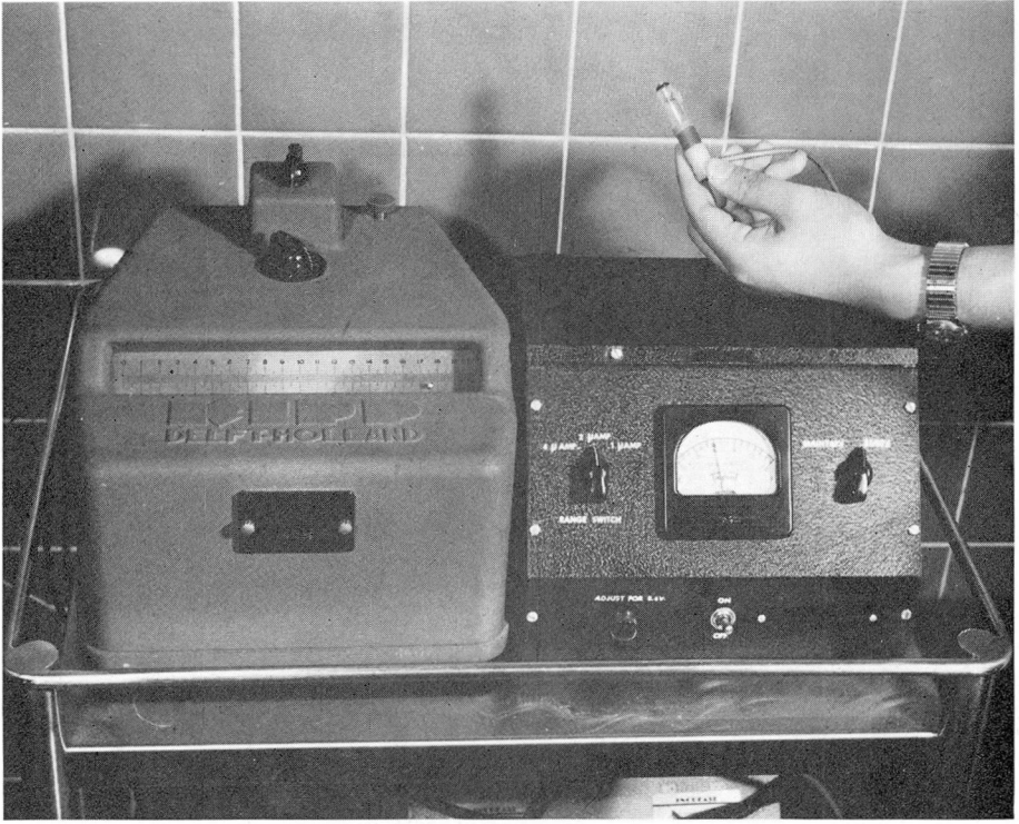
Fig. 2. Photograph of the Clark electrode with its polarograph and galvanometer. The electrode is covered with polyethylene membrane and is fixed in the oxygenator near the outflow end.
